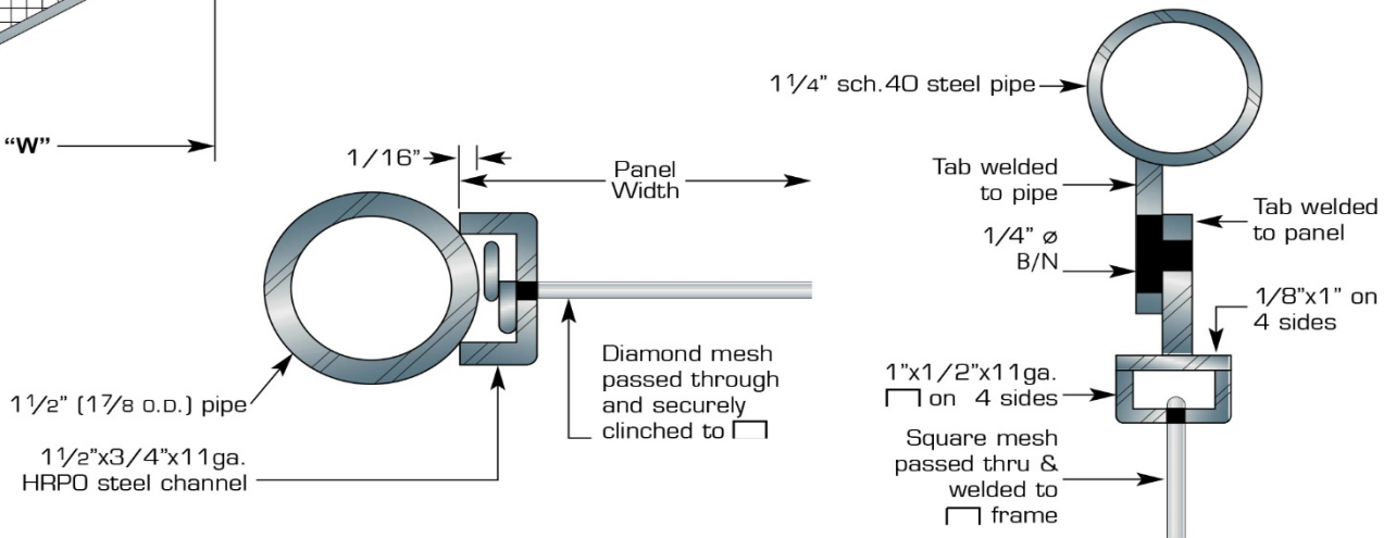
Detail of Mesh Panel Attached Directly to Pipe
